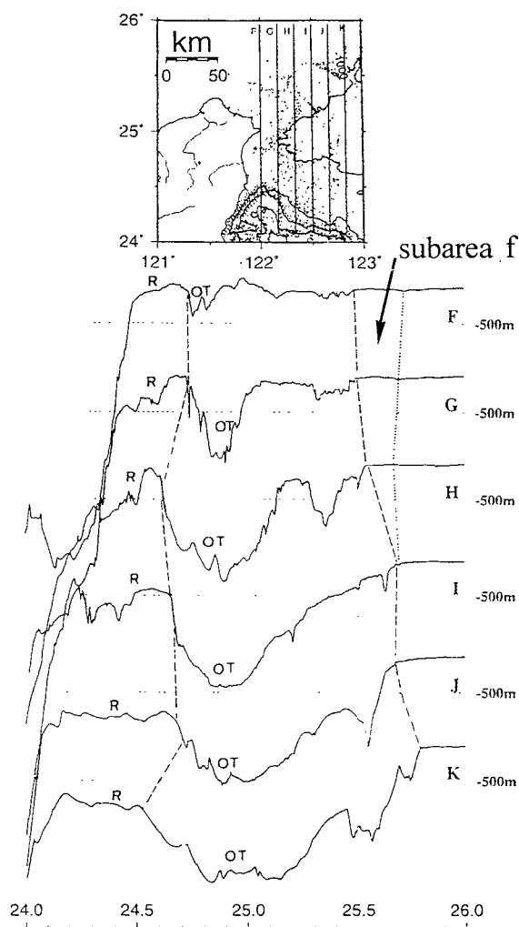
Fig. 6. The bathymetric profiles in the N-S direction near the western end of the Okinawa trough. R: Ryukyu ridge; OT: traditionally recognized Okinawa trough; Dashed lines: distinguishable boundary lines of the Okinawa trough; Dotted line: northern boundary line of subarea f (see text for explanation).
