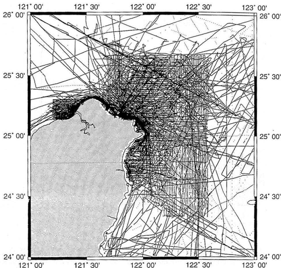
Fig. 3. Cruise lines of research vessels for the period 1990-1996 along which the bathymetric data were used for mapping the bathymetry used in this study.
