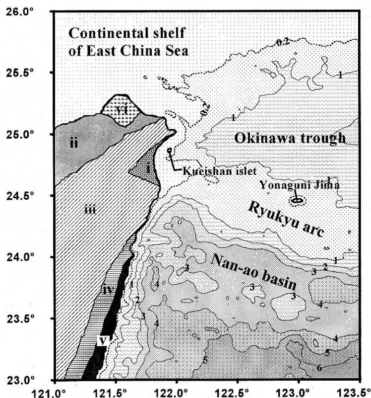
Fig. 2. Structural provinces on the Taiwan island (simplified from Ho, 1988) and its northeastern offshore area, to facilitate the discussion in the paper. The bathymetric data are taken from Liu et al. (1996). i: Ilan plain; ii: West Foothills; iii: Central Range; iv: Longitudinal Valley; v: Coastal Range; vi: Tatun Volcano.
