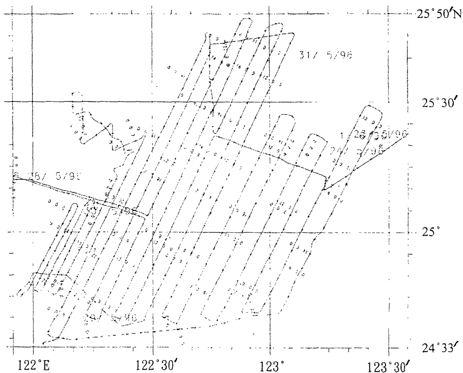
Fig. 4. Cruise lines of French R/V L'Atalante in 1996 in the westernmost part of the Okinawa trough (Lallemand et al., 1996). The cruise lines were designed to have a good coverage of the sea floor by the multi-beam echo sounder.
