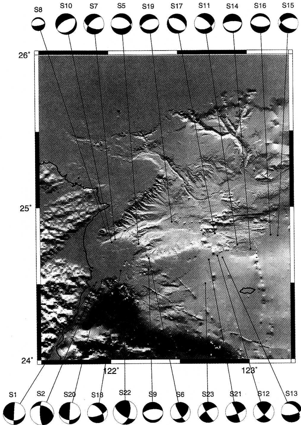
Fig. 10. Focal mechanisms of earthquakes in the western Okinawa trough (see Table 1 and text for references). Note that most of focal mechanisms in the central part of the Okinawa trough are of the normal fault type.
