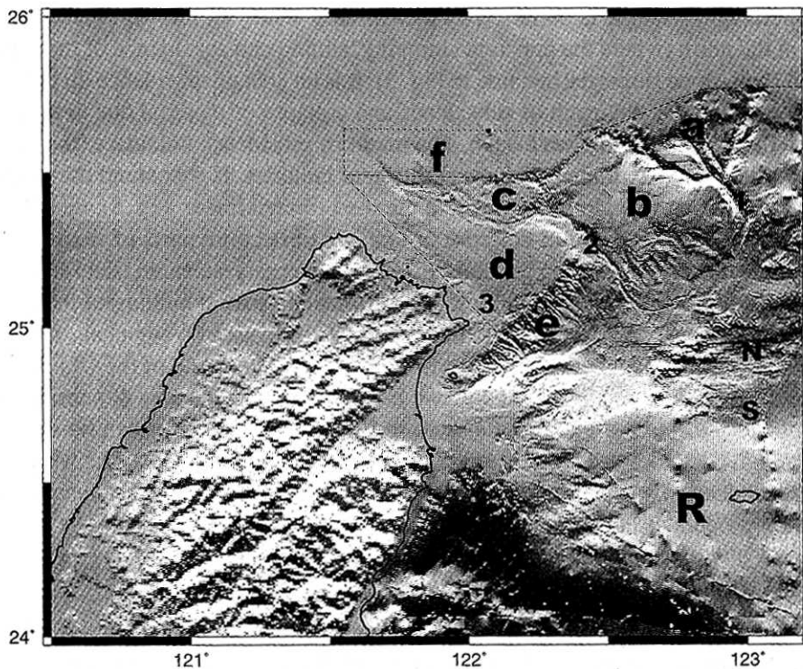
Fig. 5. Morphological map of the northeastern area of Taiwan. a: North Mien-hua Drainage Basin; b: Mien-hua Slope; c: Mien-hua Drainage Basin; d: Chilung Shelf; e: Chilung Slope; f: area for future collapsing; N: northern central graben in the deepest part of Okinawa trough; S: southern central graben; R: Ryukyu arc; 1: North Mien-hua Canyon; 2: Mien-hua Canyon; 3: Chilung Valley.
