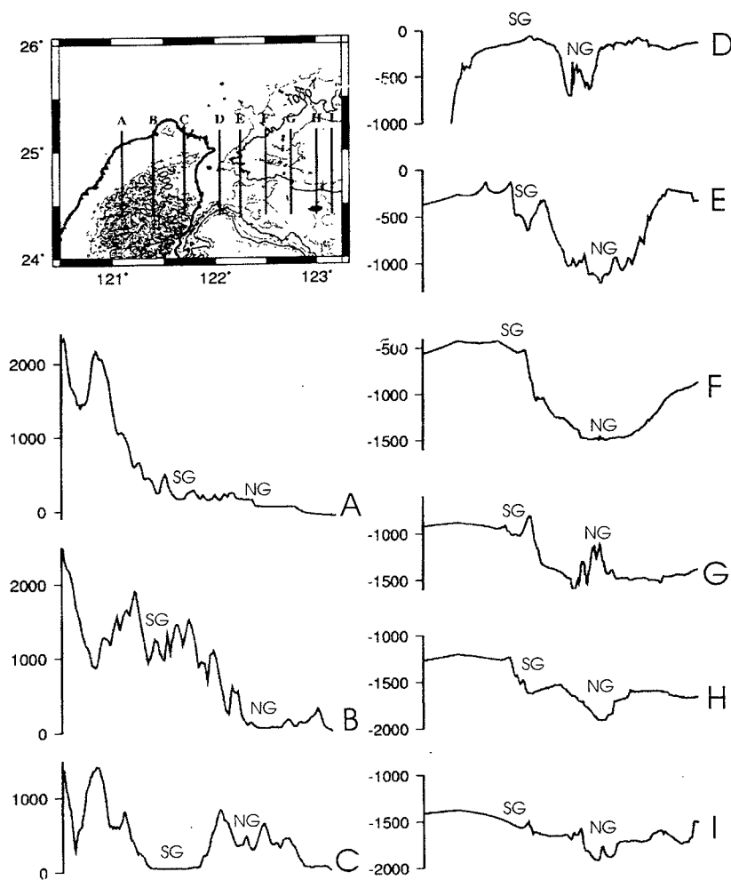
Fig. 7. The morphological profiles in the N-S direction in the northern offshore and onland areas of Taiwan for tracing the westward extension of the central grabens of the Okinawa trough. NG: northern graben; SG: southern graben.
