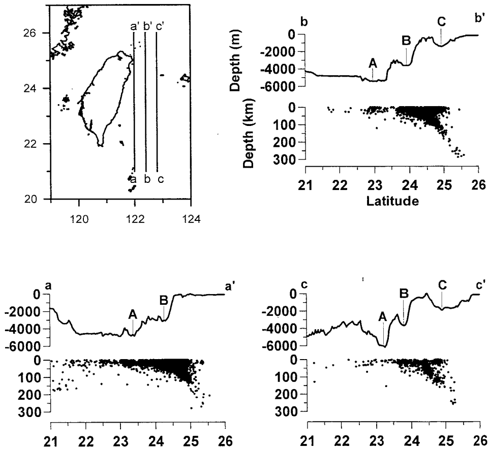
Fig. 9. The comparison of the hypocentral profiles with bathymetry in the eastern offshore area of Taiwan. The hypocenters of earthquakes shown in the profiles are within 0.1 degree on both sides of the N-S directional lines shown on the top-left corner of the figure. A: Ryukyu trench; B: Nan-ao basin; C: Okinawa trough.
