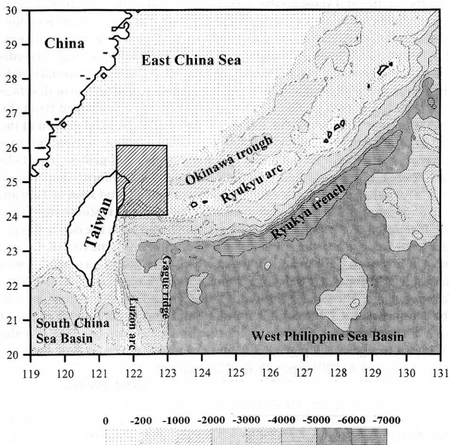
Fig. 1. The study area of this paper (box in the northern Taiwan area), with the bathymetry and tectonic units around Taiwan and in the Ryukyu subduction zone as background.
