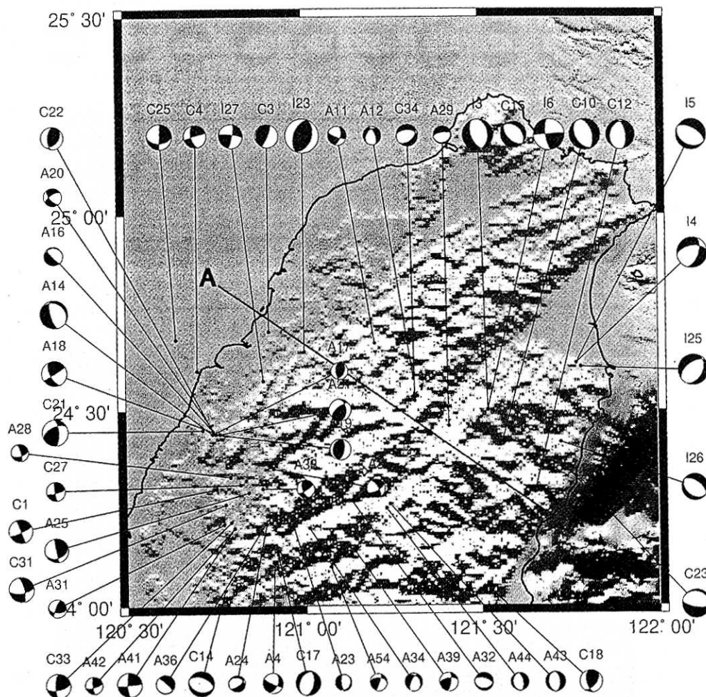
Fig. 11. Focal mechanisms of earthquakes in northern Taiwan. (see Table 2 and text for references). Note that most of the focal mechanisms are of the normal fault type and strike-slip fault type, and that most of the focal mechanisms to the north of line AA' are of the normal fault type.
