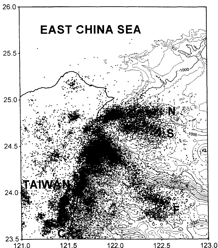
Fig. 8. Distribution of earthquake epicenters in the northeastern area of Taiwan with the bathymetric background of contour spacing of 250 meters. The Okinawa Trough Seismic Zone is divided into two E-W trending seismic belts designated by N and S. The Nan-ao Basin Seismic Belt and Northeastern Coast Seismic Zone are designated by F and C, respectively.
